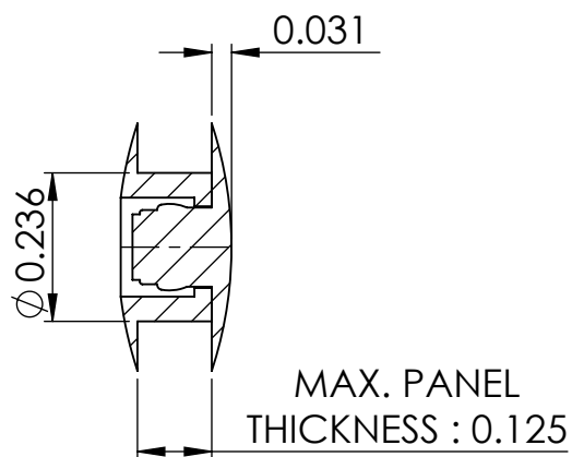
SECTION Y-Y
