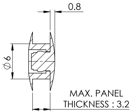
SECTION Y-Y
